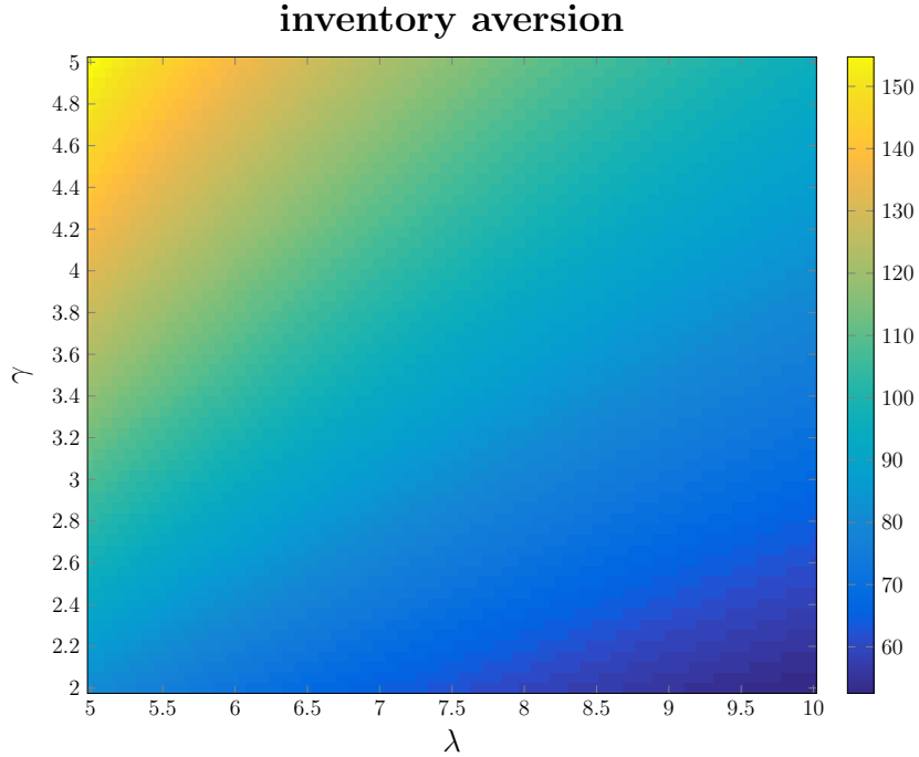
Figure 1: Inventory aversion as a function of \lambda and \gamma , when r = 0.05 , \sigma_D = \sqrt{2000} , m(\lambda, \lambda') = 2\lambda \frac{\lambda'}{\Lambda} , \lambda \sim U[5, 10] , \gamma \sim U[2, 5] , and \lambda and \gamma are independently distributed.
